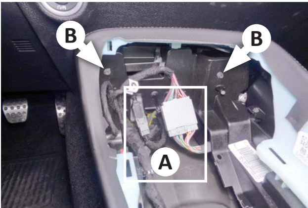
16. Separate the 2 electrical connectors (A). Then remove the 2 screws (B) at the front of the console base.
