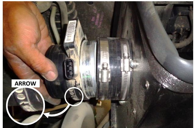
17. Install the MAF sensor in the coupling so that the airflow arrow points away from the heat shield. Push the sensor fully into the coupler, then tighten the clamp.
