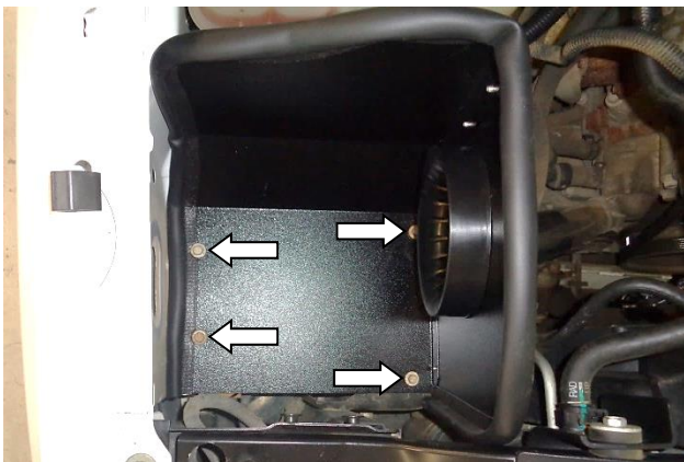
15. Use the 4 bolts removed at Step 12 to install the assembled heat shield in the vehicle. NOTE: Be sure to use the correct length bolt at each location, as determined at Step 12.
