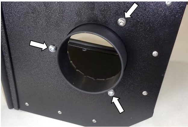
14. Attach air filter adapter (3) to heat shield using M6 screws (8), lock washers (7) and flat washers (6).
