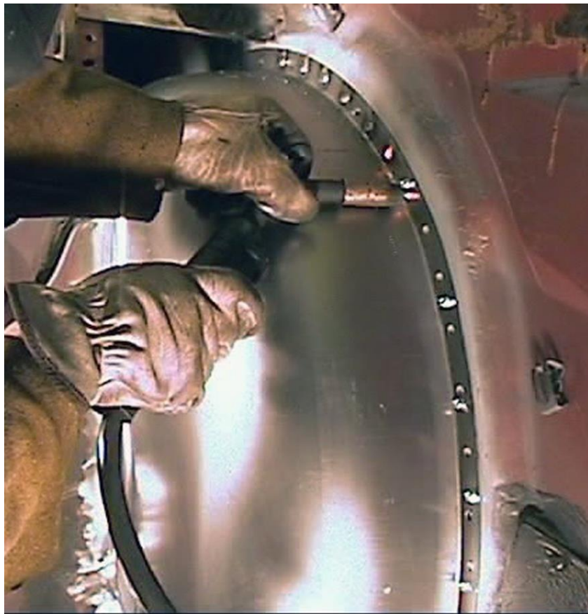
Figure 17 – Plug Weld
