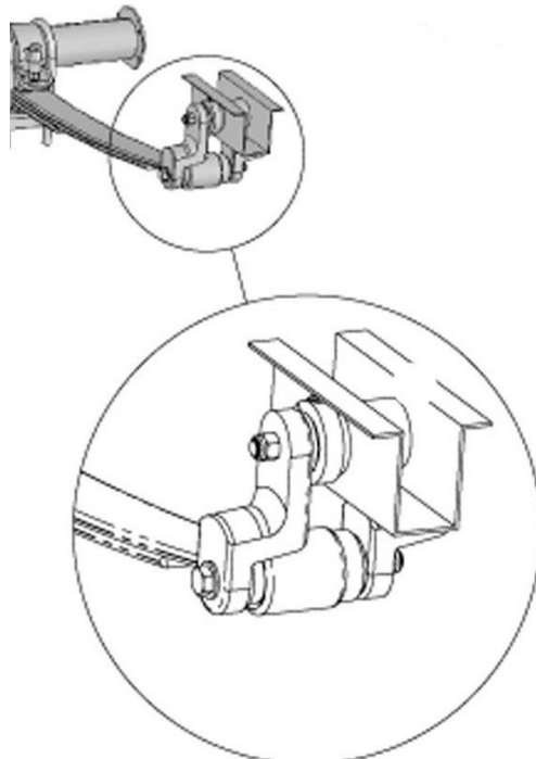
Figure 1 - Offset Shackles
