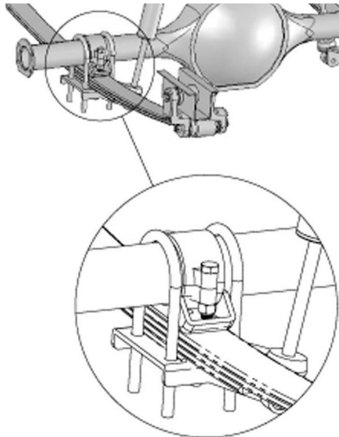
Figure 1 – Adjustable Leaf Spring Pads
