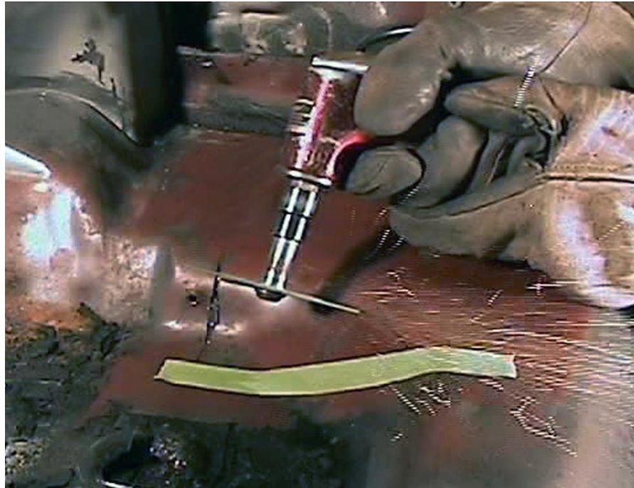
Figure 7 - Cutting for the Leaf Spring Pocket
