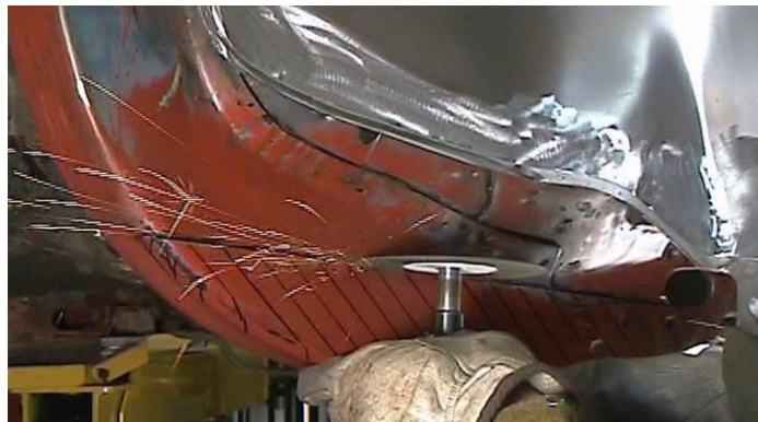
Figure 5 - Cutting the Frame Rail
