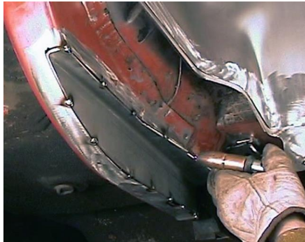
Figure 9 - Frame Rail Closeout
